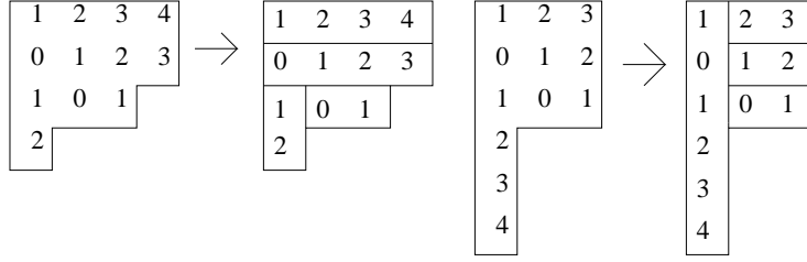
FIGURE 3. Examples: \mathcal{S}_1(1344) = (244, 2) and \mathcal{S}_1(1^3 3^3) = (222, 6)
